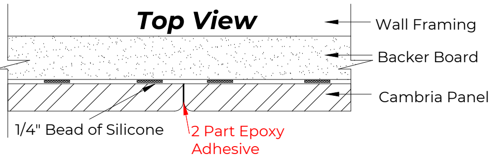
Hard Seam "Half Round" Joint
