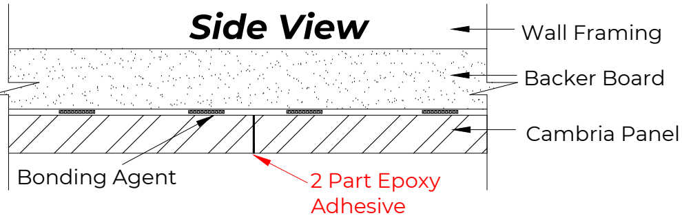
Hard Seam Butt Joint
